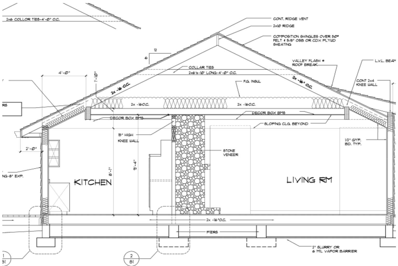
1 CROSS SECTION 3/8"=1'-0"
